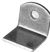
JCRC8S 1-1/2" x 1-1/2" 9 Ga, Hole: 3/8"
